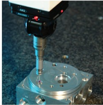
High accuracy TP200 touch trigger probe
