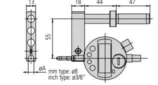
12AAA837 Dial indicator (ø3/8" stem) holder
